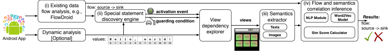
Figure 2: FlowCog Architecture
