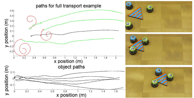
Figure 8: (Upper left) The paths of three robots (red during phase 1 and green during phase 2) and object (black). (Lower left) The path of object center-of-mass over five trials. (Right) Image of robots in starting position, after attachment, and after transport. For all cases, the goal is on the right.
