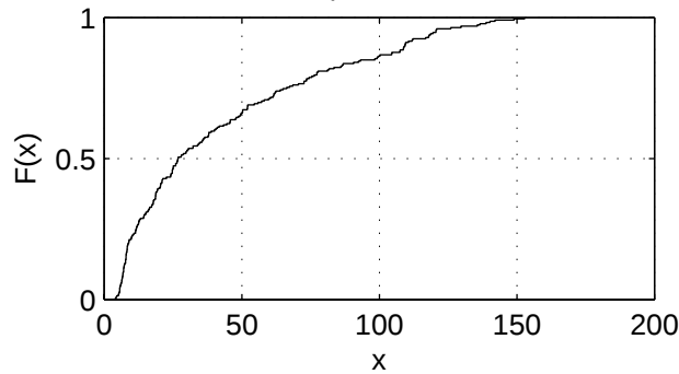
Empirical CDF
