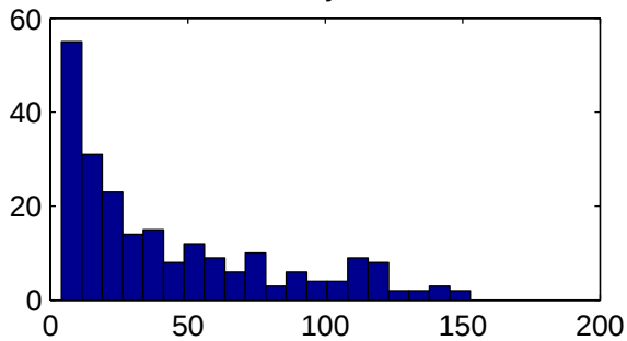
226 samples
