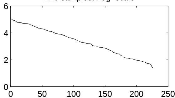
Empirical CDF
