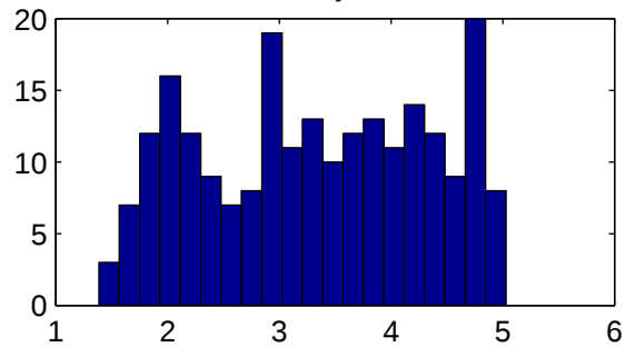
226 samples, Log-scale
