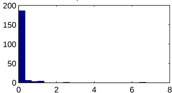
201 samples
