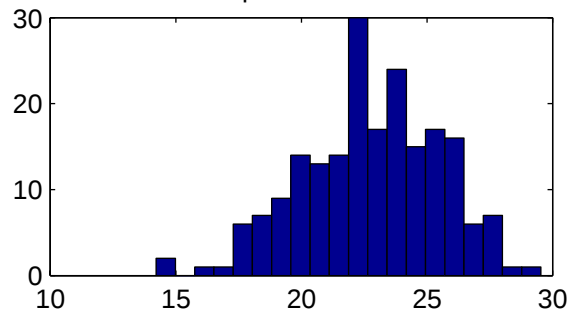
201 samples, Log-scale
