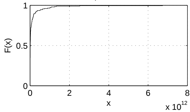
Empirical CDF
