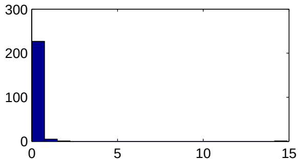
234 samples
