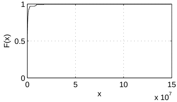
Empirical CDF
