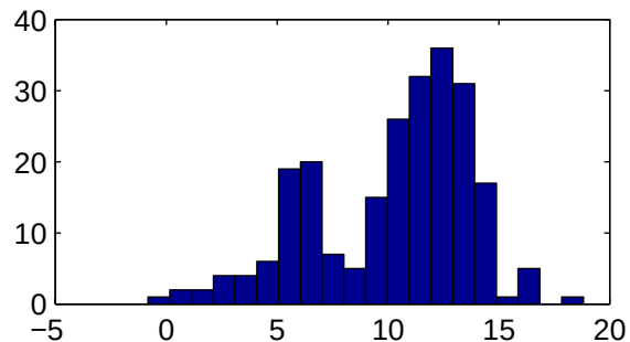
234 samples, Log-scale
