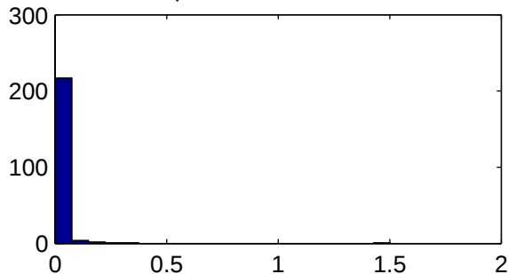
226 samples
