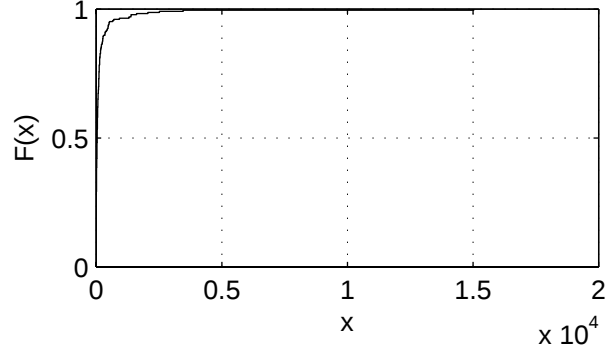
Empirical CDF
