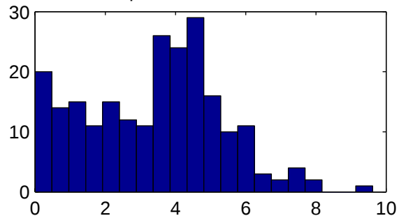
226 samples, Log-scale
