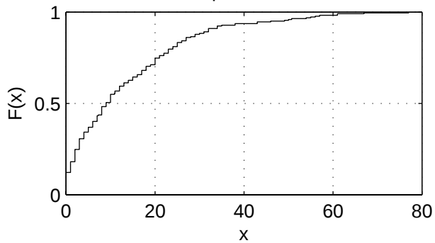
Empirical CDF
