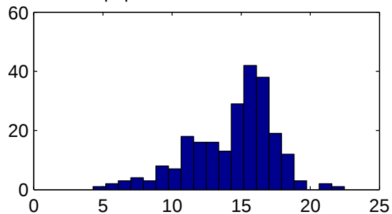
237 samples, Log-scale
