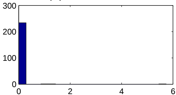
237 samples
