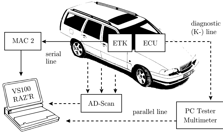
Figure 8.3: Architecture for data acquisition in the demonstrator car
