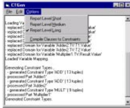
Figure 7.3: Screenshot of the System Description Generator (generating a system description for the pedal position sensor)
