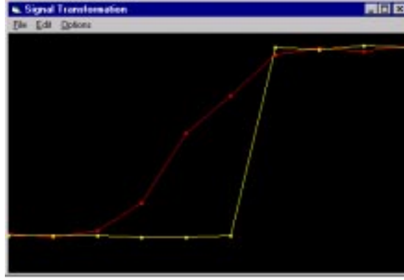
Figure 7.7: Example of Measurements for the Pedal Position Sensor (darker line shows signal of v_{pos} , brighter line shows signal of v_{switch} )
