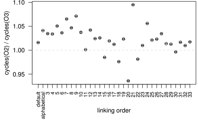
(a) Perlbench
