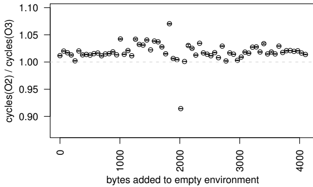
(a) Perlbench
