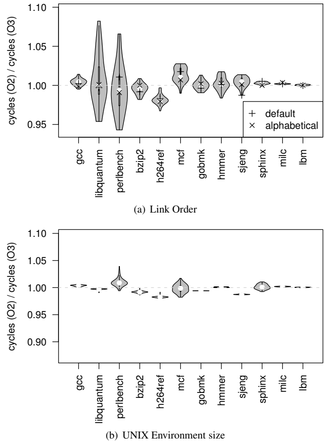
Figure 4. Bias in Intel’s C compiler on Core 2.
