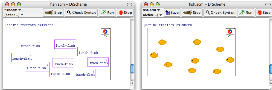
Fig. 4. A pict box containing Scheme boxes
