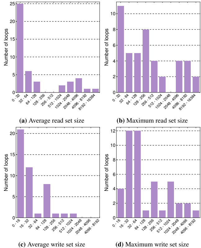
Figure 12: Histograms of average/maximum read/write set sizes (in bytes) show that a transaction can be accommodated by contemporary hardware supports.
