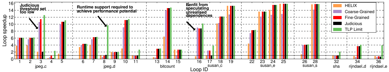
Figure 10: Performance obtained with hardware transactional memory. Fine-grained speculation with hardware support approaches the theoretical maximum speedup. Loops which showed no potential for speedup with the TLP limit model have been removed for clarity.
