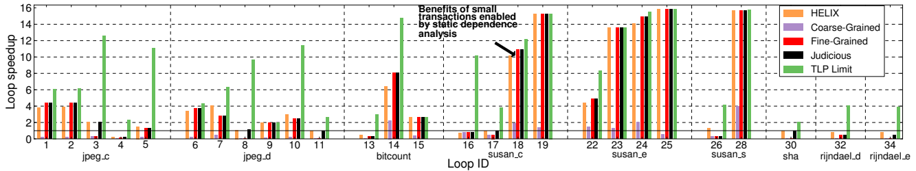
Figure 11: Performance obtained with software transactional memory. While all speculation models have lower performance compared to when hardware transactional memory is used, the coarse grain speculation model performs worst.
