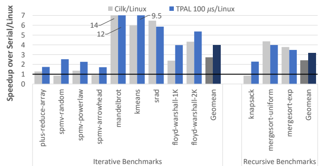
Figure 7. Speedups over serial execution on Linux, 15 cores. Overall TPAL outperforms Cilk Plus.
